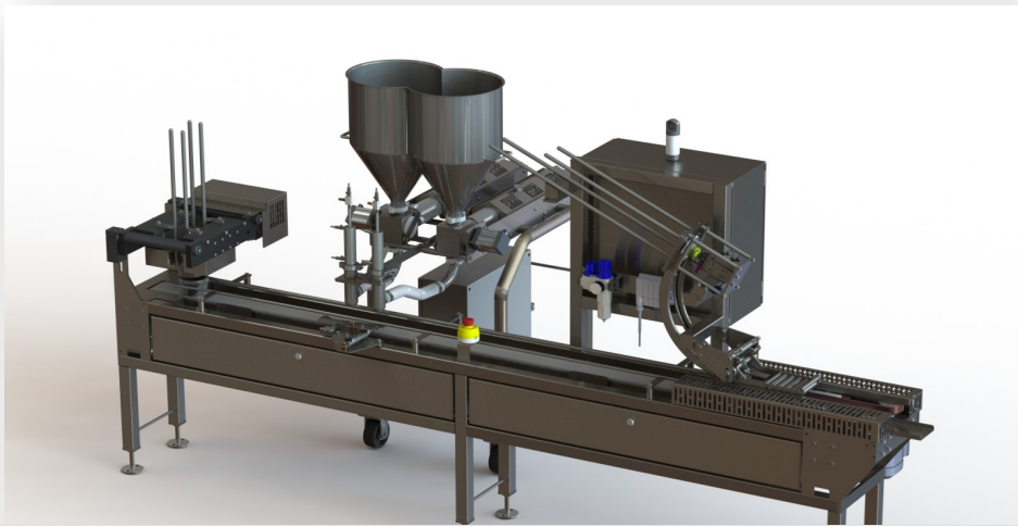
SALSA PACKAGING SYSTEM Two Head Piston Filler Shown over a Precision PMD DNester and Lid Applicator for Salsa. System speed is 50 cups per minute (16oz fill).
